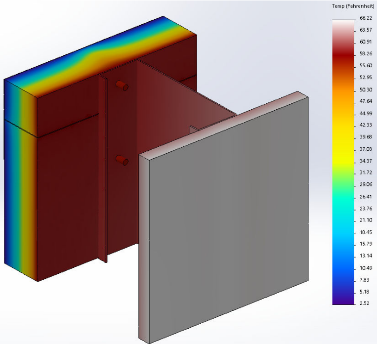
Exterior continuous insulation, with 2" polyisocyanurate, 1/32" gap between insulation panels Exterior temperature 0°F / Interior temperature 70°F Contact resistances & air film coefficients were incorporated in the model
