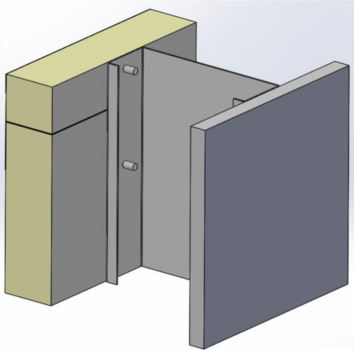
Exterior continuous insulation, with 3" polyisocyanurate, 1/32" gap between insulation panels Exterior temperature 0°F / Interior temperature 70°F
