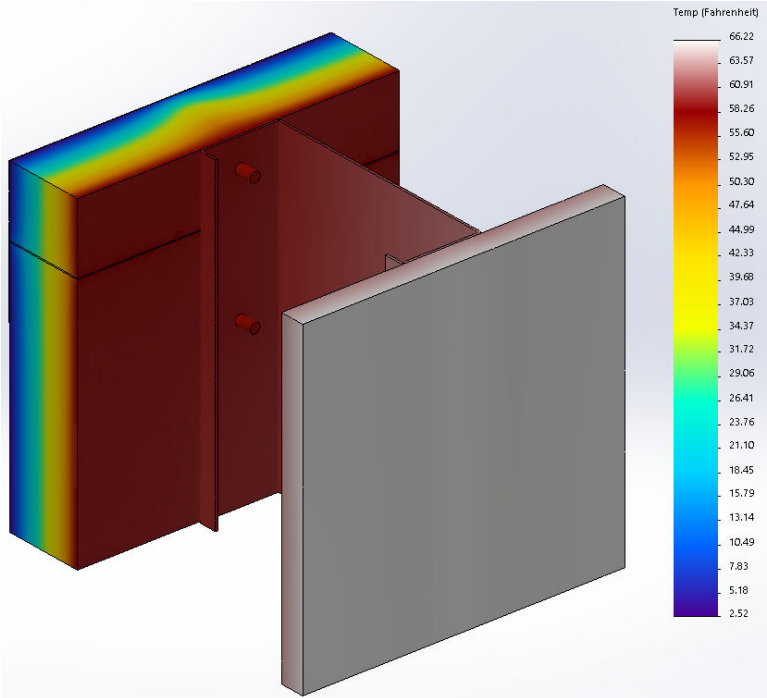
Exterior continuous insulation, with 3" polyisocyanurate, 1/32" gap between insulation panels Exterior temperature 0°F / Interior temperature 70°F Contact resistances & air film coefficients were incorporated in the model
