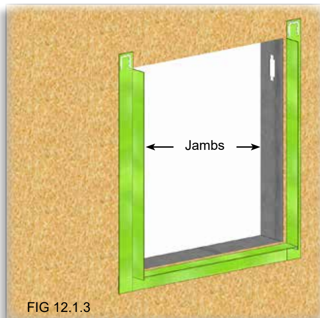
2-Jambs: Using an appropriately sized piece of the SMARTci Trim, ship lap the jamb pieces of trim over the trim at the sill. Place a bead of sealant at the underside of each corner. Place a 1/4" (min.) horseshoe-shaped bead of sealant where the jamb trim will ship lap with the header. Attach to substrate as required. Reference details beginning on page 28.
