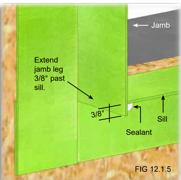
4-Corners: Overhang sill and jamb trims as shown above and in the breakout box on page 23. A 1/4" (min.) bead of sealant should be placed along the underside of all four corners. Reference details beginning on page 28.
