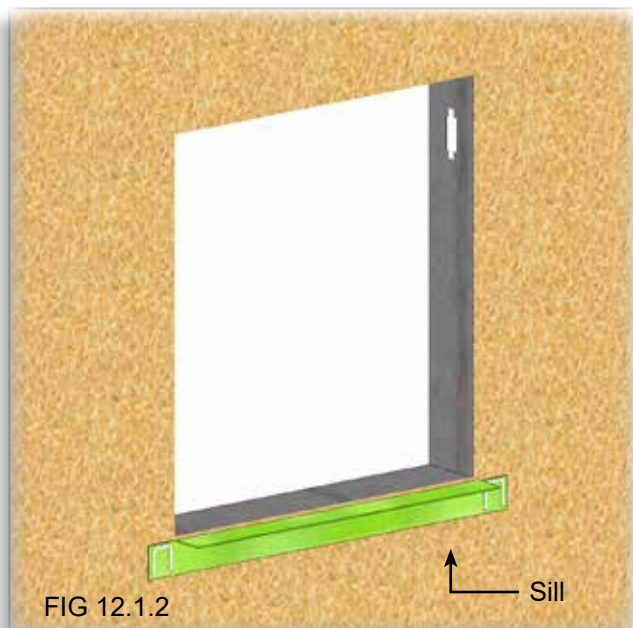
1-Sill: Using an appropriately sized piece of the SMARTci Trim, place the trim as shown above to allow for the ship lap of each jamb trim. Place a 1/4" (min.) horseshoe-shaped bead of sealant as shown prior to shiplapping jamb trim. Attach to substrate as required. Reference details beginning on page 28.
