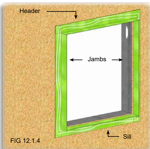
3-Header: Using an appropriately sized piece of the SMARTci trim, ship lap the header piece of trim over the trim at the jamb. Place a 1/4" bead of sealant at the underside of each corner. Attach to substrate as required. Add two 1/4" (min.) continuous beads of approved sealant as shown prior to installing insulation (optional for 2.5-in-1 system). Reference details beginning on page 28.
