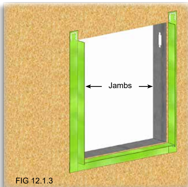
2-Jamb: Using an appropriately sized piece of the SMARTci Trim, ship lap the jamb pieces of trim over the trim at the sill. Place a bead of sealant at the underside of each corner. Place a 1/4" (min.) horseshoe-shaped bead of sealant where the jamb trim will ship lap with the header. Attach to substrate as required. Reference details beginning on page 28.
